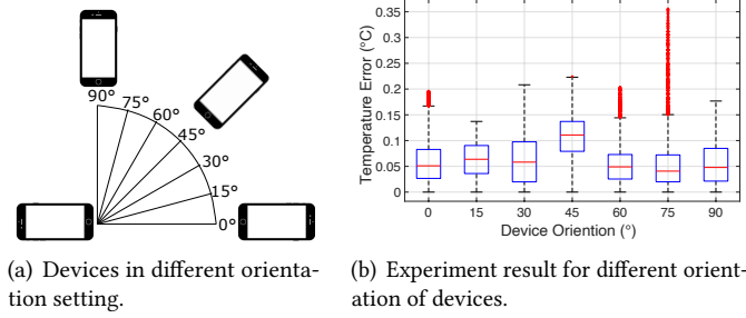
Fig. 16. Experiments on device orientation.
